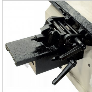
Tilt Fence Adjustment
