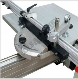
Material Clamp with Adjustable Guide
