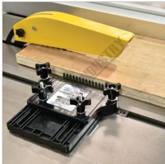
In Use Tabel Saw
