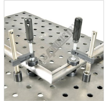
Round Tube Setup with Clamps and Optional V Pads
