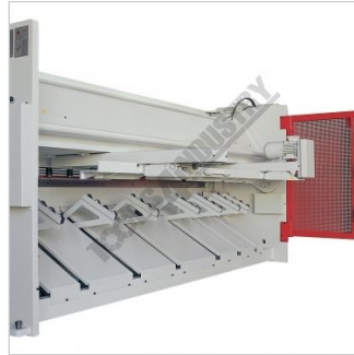
Pneumatic Sheet Supports Type A
