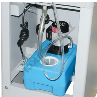
Coolant System
