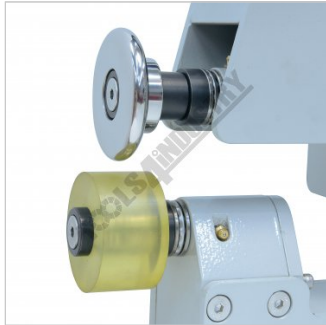
Polyurethane Lower Wheel with 3/8 Inch Tipping Die
