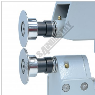
Outside Offset Die with Knife Edge Tipping Die
