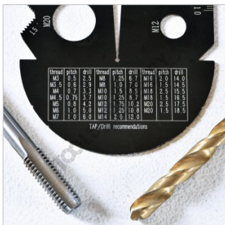
Tap-Drill Chart
