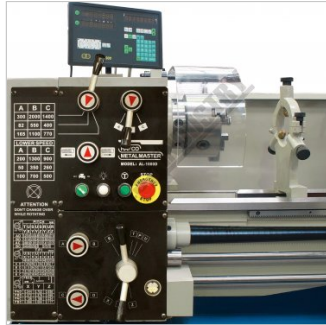
Headstock Controls
