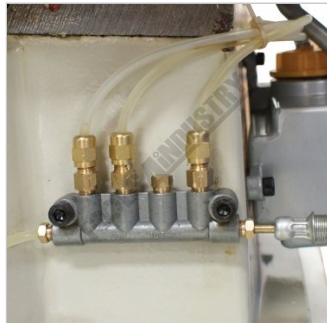
Lubrication directional Housing Block
