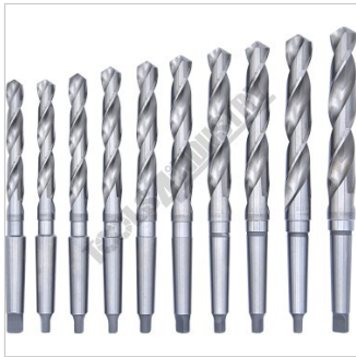
Metric 2MT HSS Drill Set
