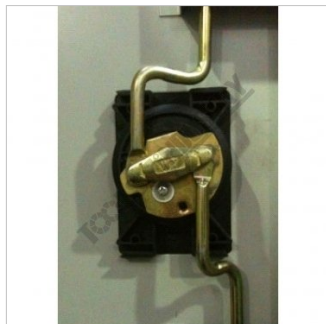
8TB0500 KEY AND LOCK CYLINDER SET.2
