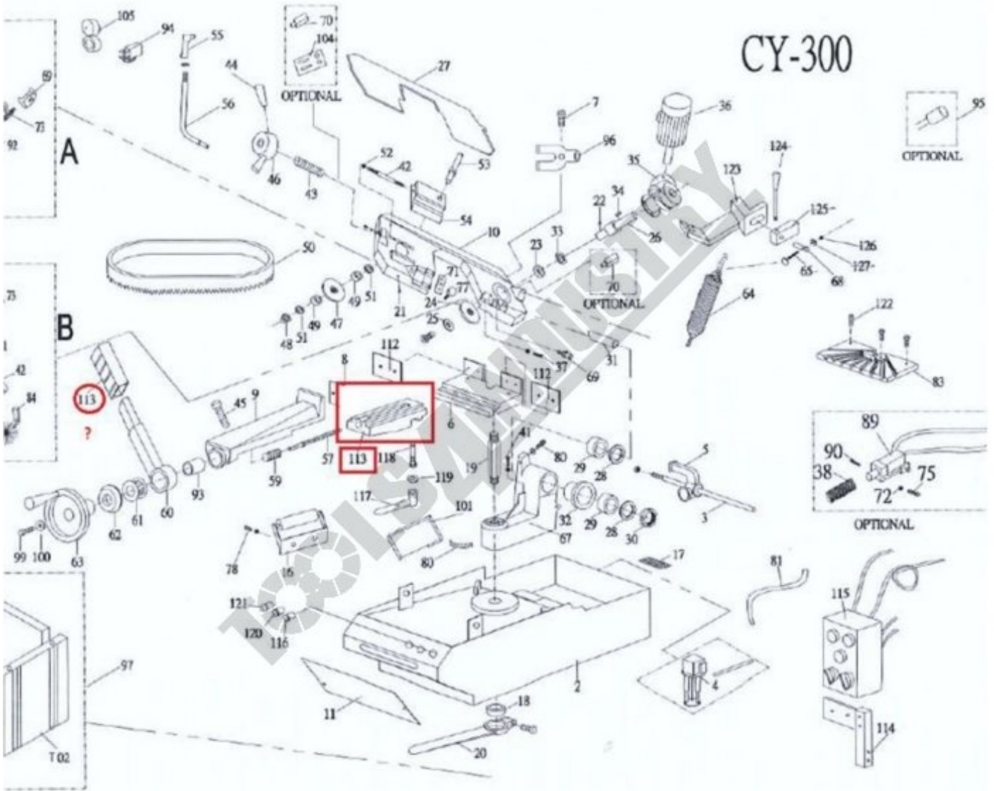
113. Vice sliding seat
