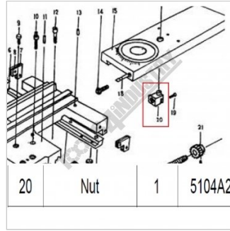
2LX5104 NUT (CROSS) 5104A2
