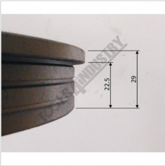
2FV0017 WHEEL OD 405 BORE 52
